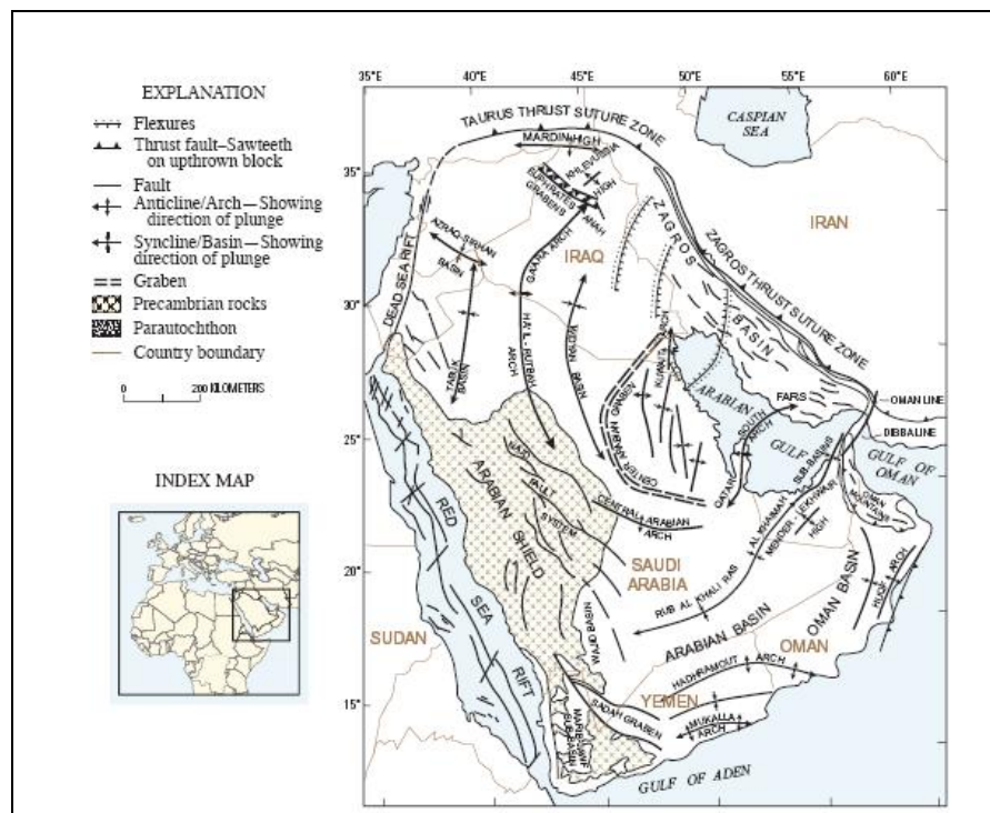
Figure 2 Tectonics and geologic structure of the Arabian plate with Zagros Folded Belt (Reported by Wassel, 2005 based on James E. Fox and Thomas S. Ahlbrandt, U.S. Geological Survey Bulletin, 2002).
