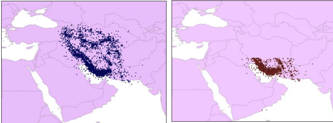
Figure 3 Seismogenic zone taken as the whole area for seismicity results from the subduction zone activity (Source I and II).
