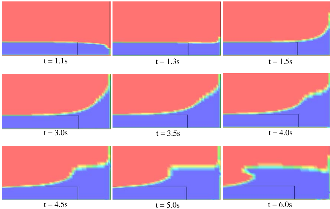
Fig. 5 Tsunami Wave Runup on a Rigid Wall
