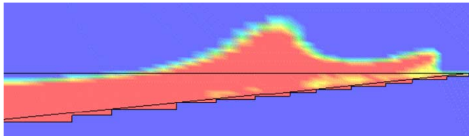
Fig. 4 Tsunami Wave Runup on a Shoreline
