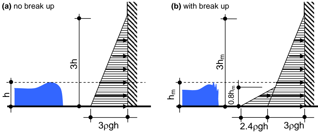
Fig. 1 Tsunami Wave Pressure Distribution with/without Soliton Break-up
