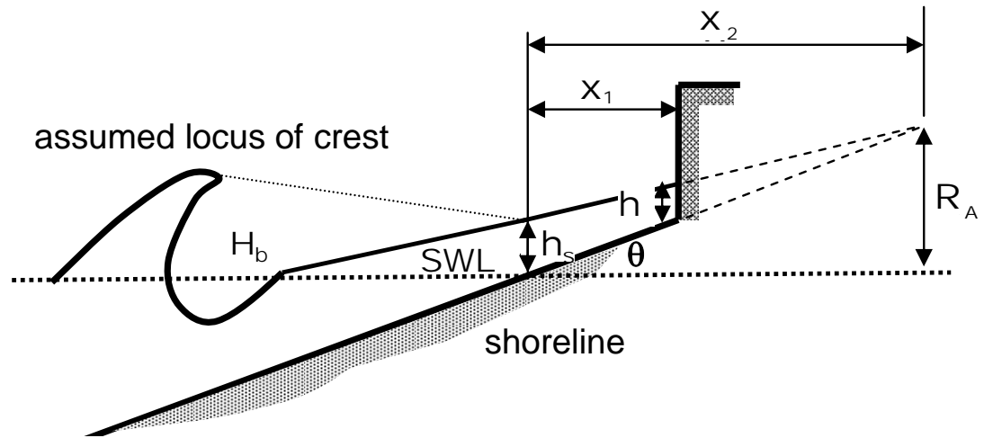
Fig. 2 Wave Pressures from Broken Waves on Walls Landward of the Still-Water Line
