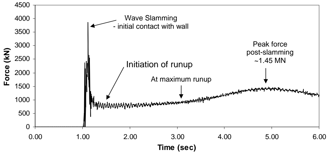
Fig. 6 Tsunami Force Time-history on a Rigid Wall
