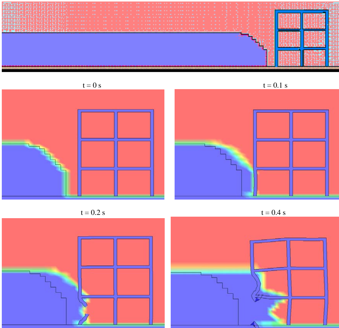
Fig. 7 Structural Damage due to a Tsunami Wave
