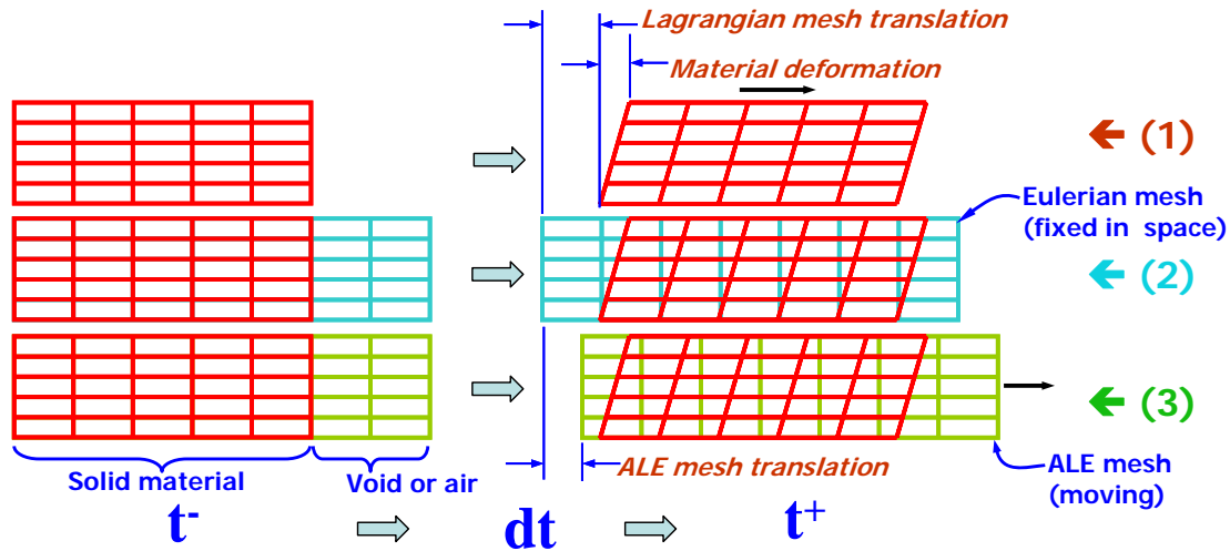
Fig. 3 Description of Arbitrary Lagrange Euler (ALE) Technique used in LS-DYNA
